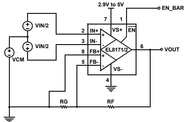
FIGURE 28. CIRCUIT 1 - GAIN IS BY EXTERNAL RESISTORS RF AND RG
