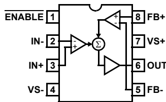
EL8171, EL8172 (8 LD SO) TOP VIEW
